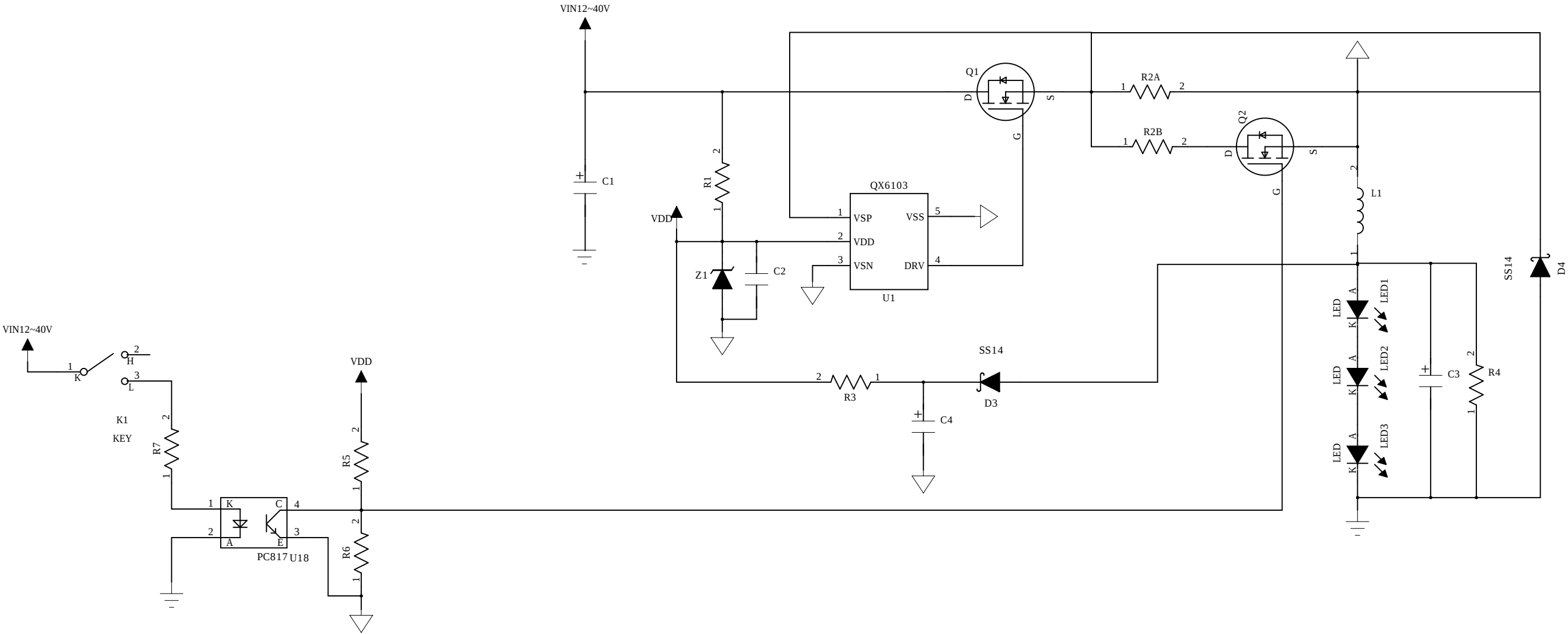
Brightness Controller
